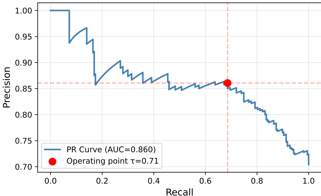
Precision-Recall: SAFE/WAIT Decision (Validation Set, n=294)
