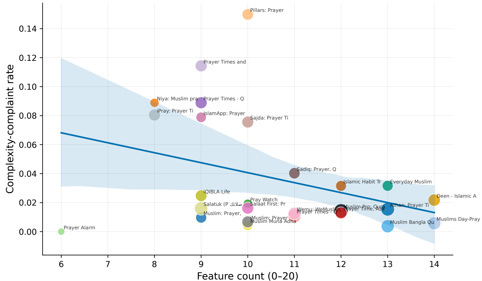
RQ5 — feature bloat vs. complexity complaints (n = 26 apps) Exploratory: app-level n is small; marker size = log review volume
