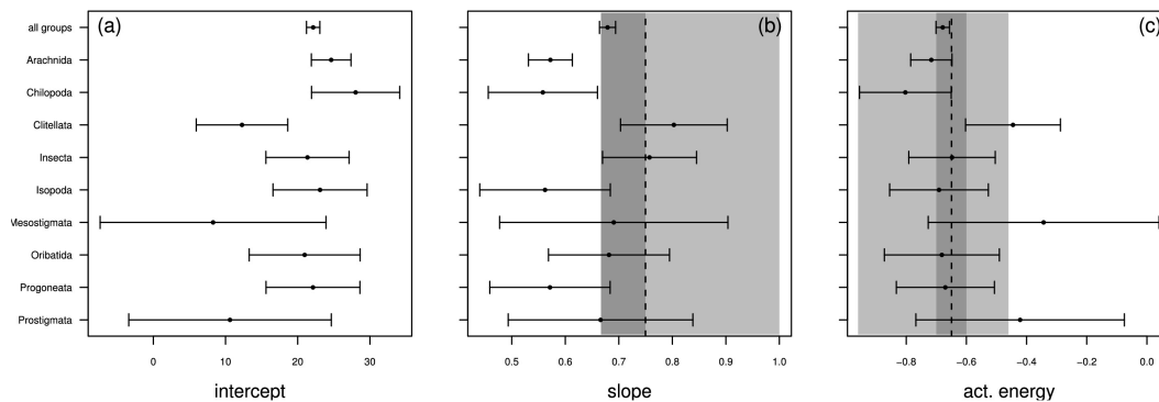
Figure 3: Distribution of fitted metabolic scaling parameters and their 95% confidence limits in the phylogenetic model across phylogenetic groups: (a) intercepts, (b) allometric exponents and (c) activation energies. Parameters of the linear model (all groups) have been included. Indications of model predictions: (b) dashed line equals 3/4 (MTE); gray and dark gray areas indicate ranges 2/3 - 1 and 2/3 - 3/4 , respectively (alternative models); (c) the dark gray area indicates range -0.6 to -0.7 eV and the dashed line the mean 0.65 eV (MTE); the light gray area depicts range -0.46 to -0.96 eV.
