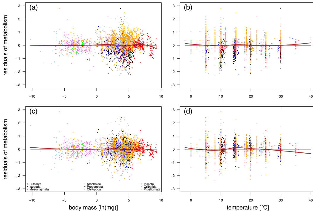
Figure 2: Accuracy of polynomial and phylogenetic models: distributions of the residuals for the polynomial (a, b) and the phylogenetic model (c, d) across the natural logarithms of body mass (a, c) and temperature (b, d). Systematic deviations of the data from model predictions are characterized by loess fits (brown curves). See Table 1 for parameters of the fitted polynomial and phylogenetic model.
