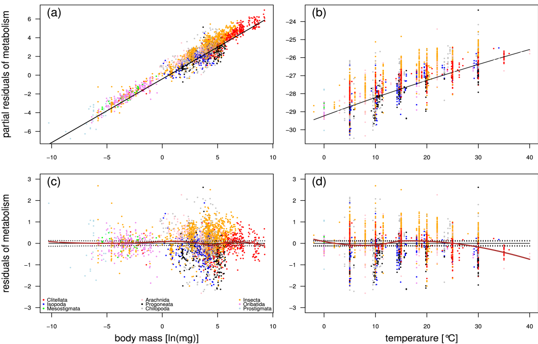
Figure 1: Metabolic scaling according to the linear model: dependence of partial residuals of the natural logarithm of metabolism on (a) the natural logarithm of body mass and (b) temperature with the fitted multiple linear model (black line). In these partial residual plots, metabolism is plotted against one of the independent variables while accounting for the effect of the other. Distributions of the linear model's residuals (deviation of data points from black line in panels a and b) across (c) the natural logarithm of body mass and (d) temperature characterized by deviations of the loess fit (brown curves) from the 95% confidence bands (dotted black bands). See Table 1 for parameters of the fitted linear model. Note that statistical fits employed inverse temperature terms, whereas figure axes were labelled with temperature.
