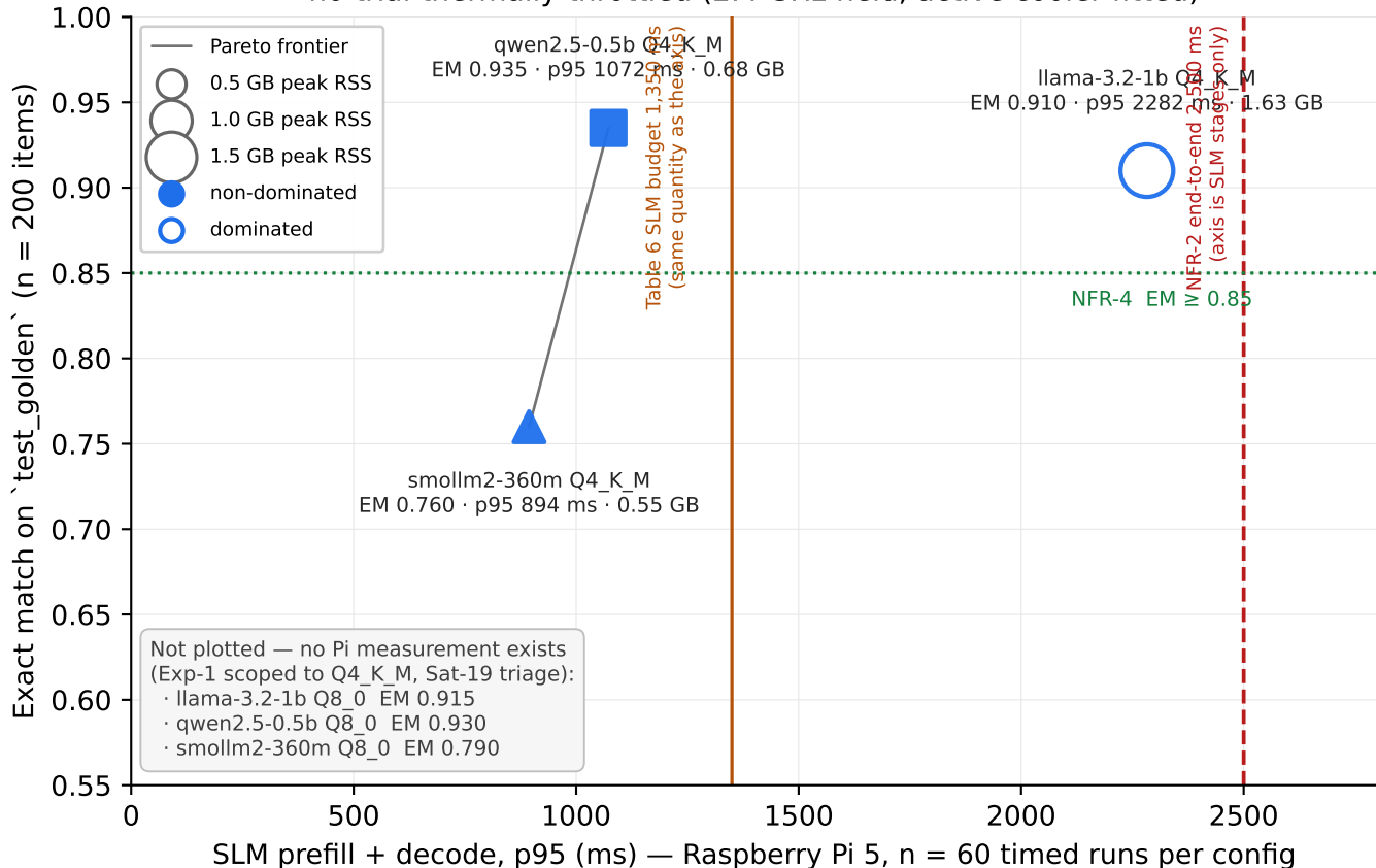
Figure 2 — Accuracy/latency Pareto frontier, Surface B no trial thermally throttled (2.4 GHz held, active cooler fitted)
