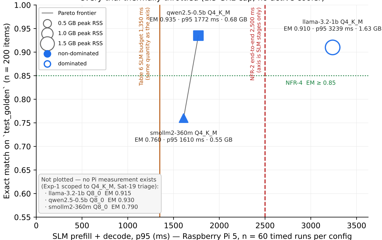
Figure 2 — Accuracy/latency Pareto frontier, Surface B every trial thermally throttled (1.5 GHz cap, no active cooler)
