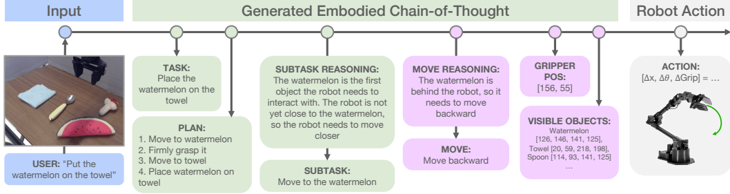
Figure 3: Steps of our embodied chain-of-thought reasoning. We interleave several intermediate reasoning steps into the mapping from inputs to robot actions. Green: standard linguistic chain-of-thought steps that break a given instruction into the required sub-tasks. Purple: Embodied chain-of-thought steps that require grounding the policy’s reasoning in the scene and robot state. Our experiments show that these grounded reasoning steps are key to improving policy performance with chain-of-thought reasoning.
