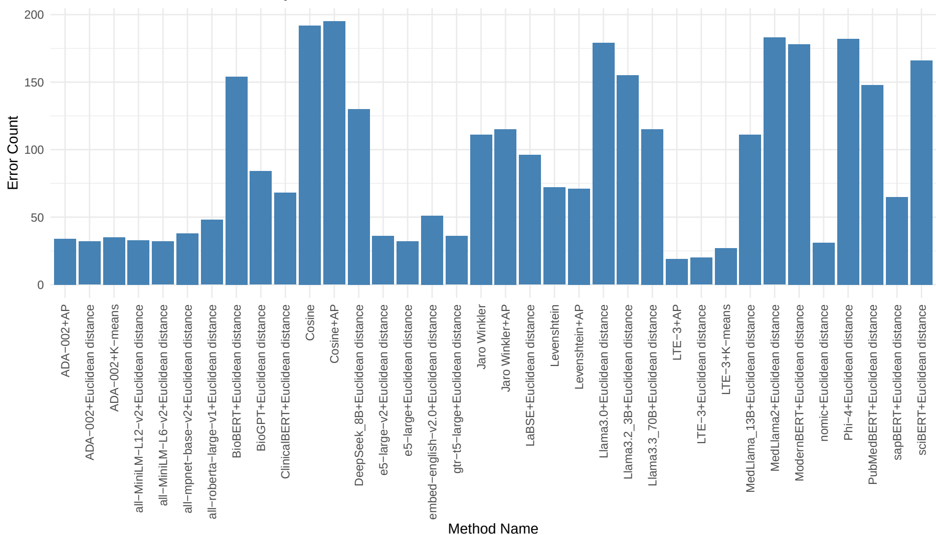
Count of Miscellaneous Error by Method, WHO-all
