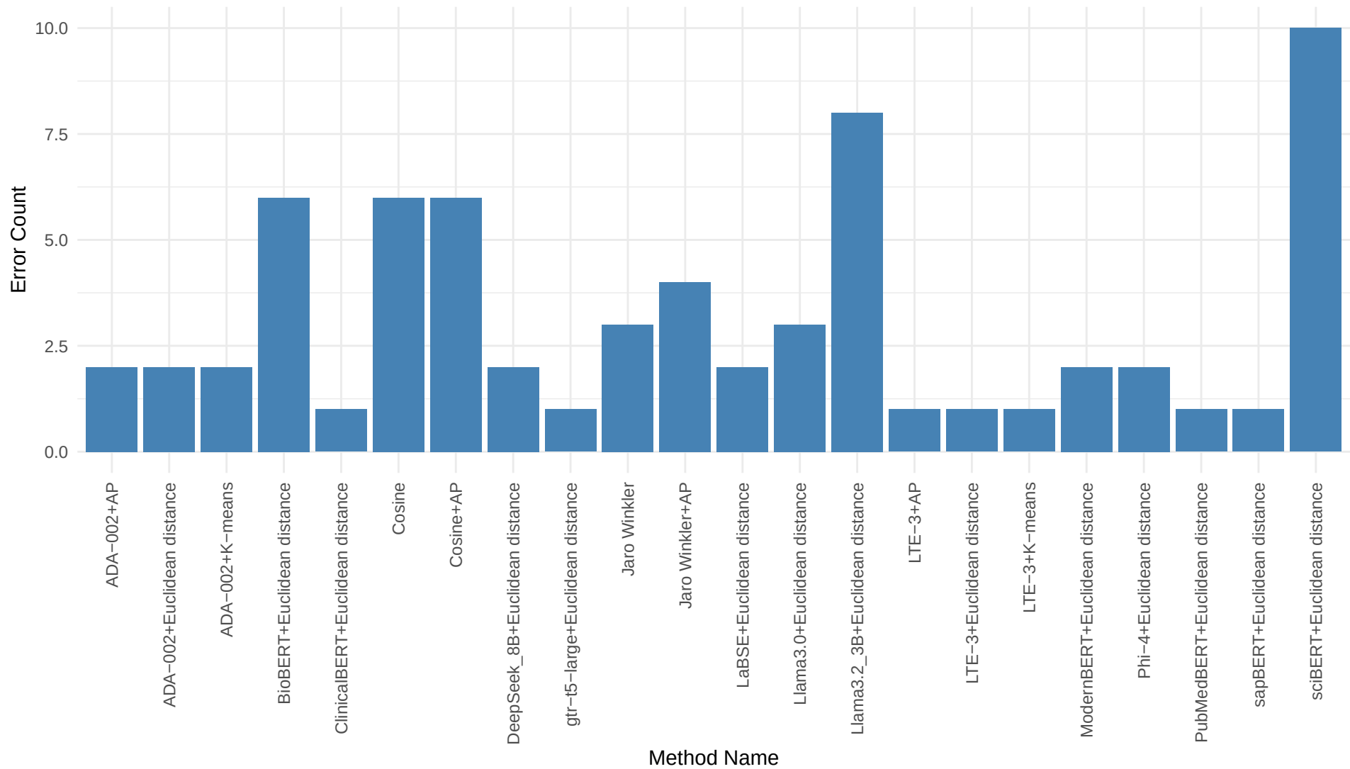
Count of Treatment-related Mismatch by Method, WHO-all
