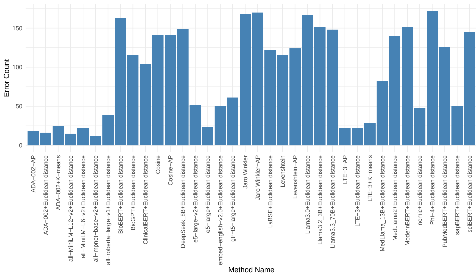
Count of Anatomical Mislocalization by Method, WHO-all
