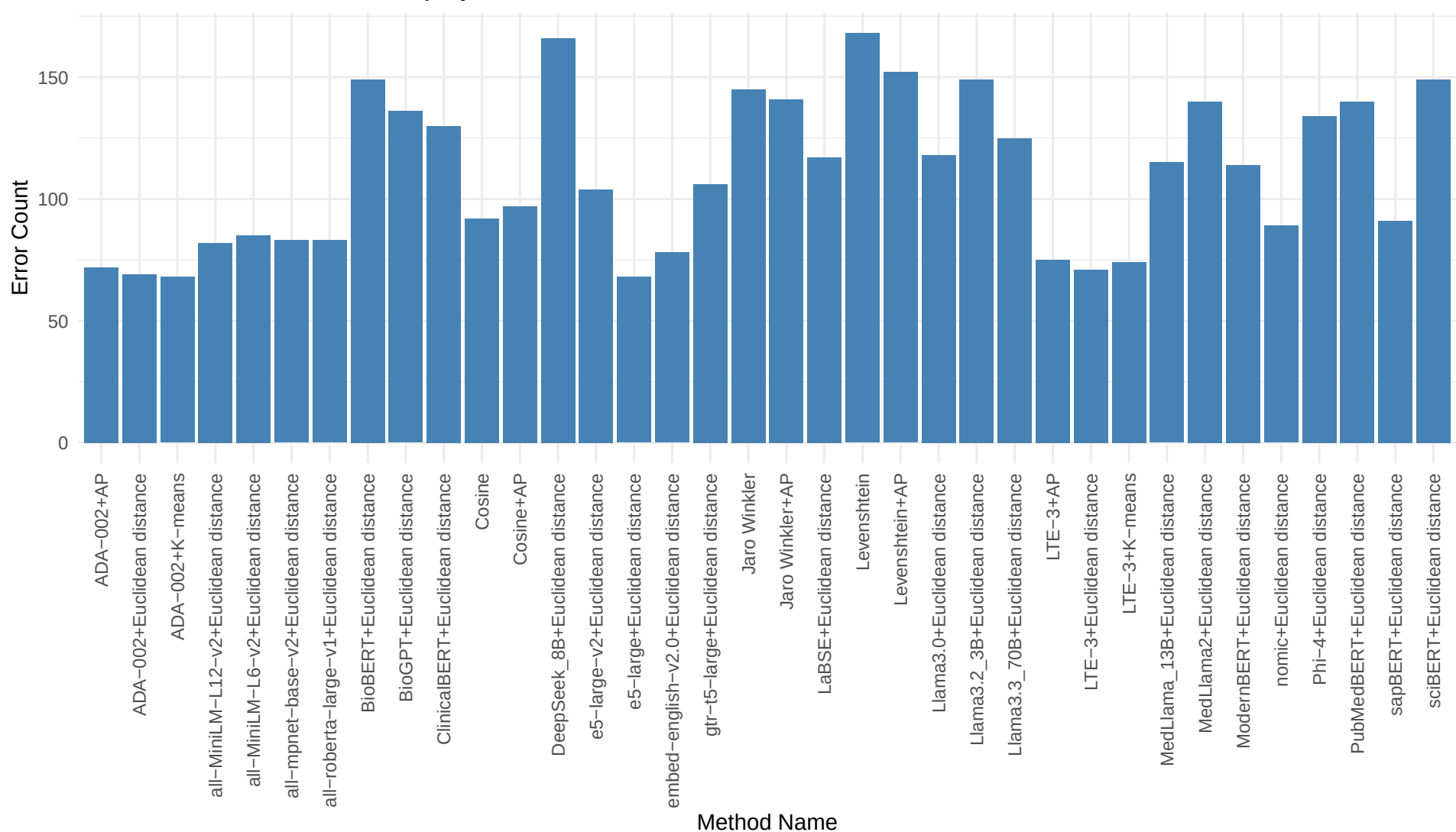
Count of Partial Name Overlap by Method, WHO-all
