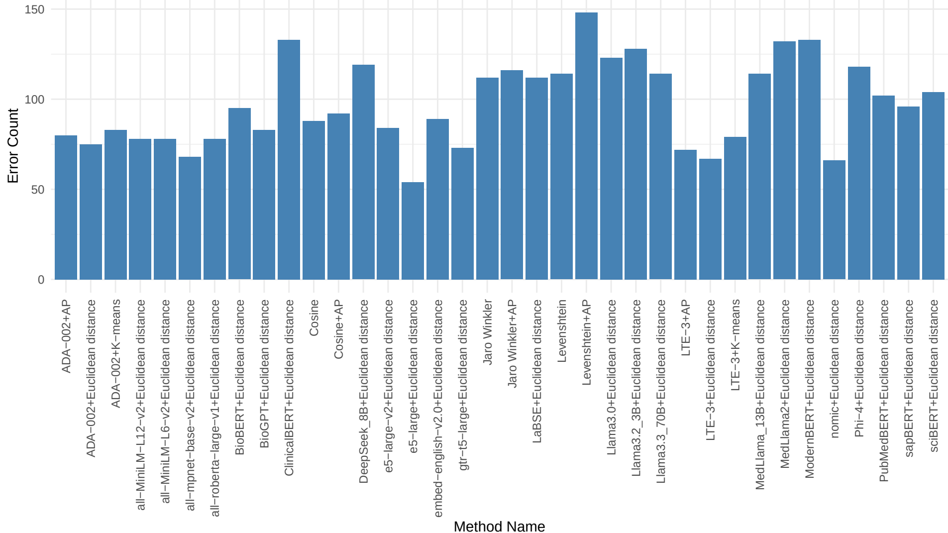
Count of Subtype/Subclass Mismatch by Method, WHO-all
