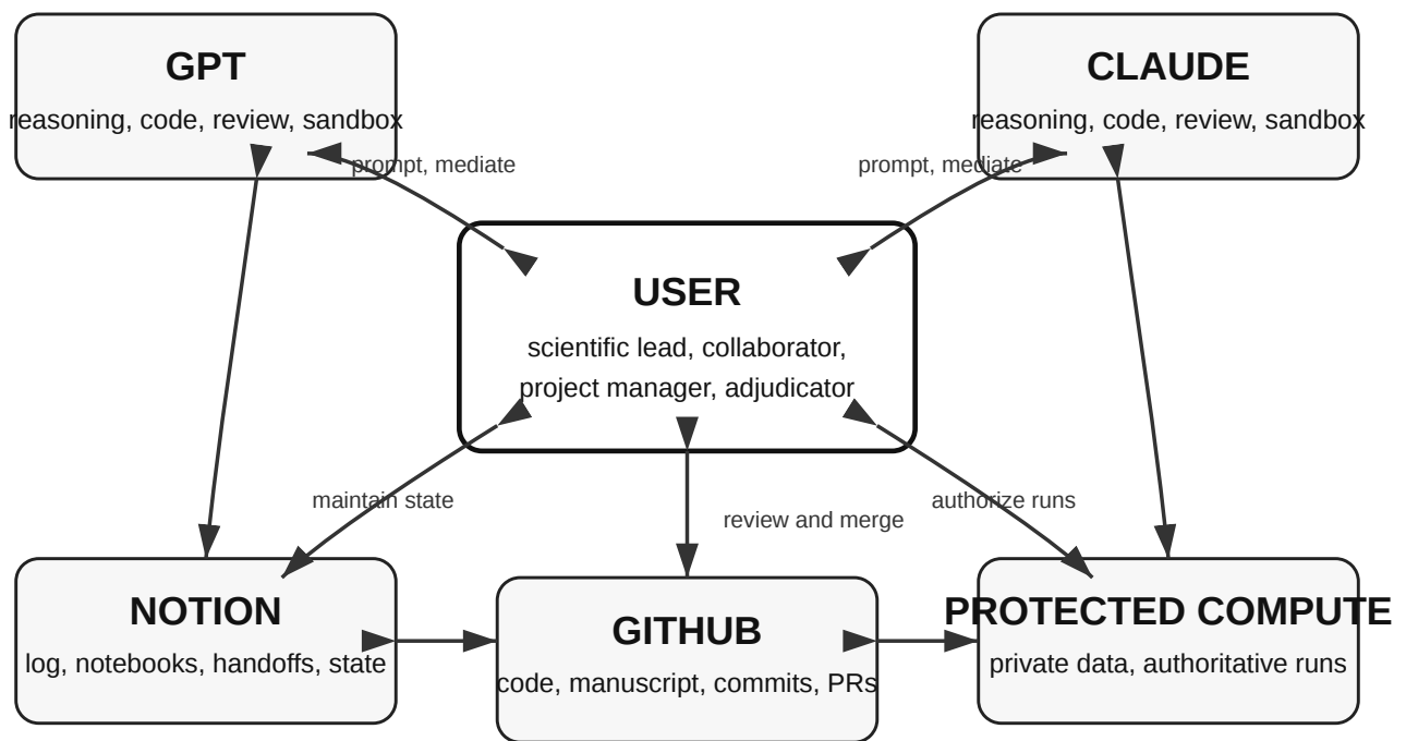
Figure 1: The User mediates the workflow. GPT and Claude read and write shared state in Notion, review versioned artifacts in GitHub, and test code in separate sandboxes. The User initiates attention shifts, controls protected execution, and accepts or rejects project state.
