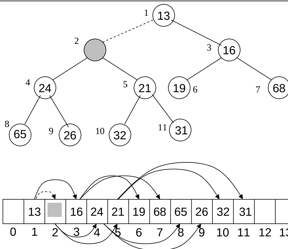
Figure 29.10: inserting new value in a heap
