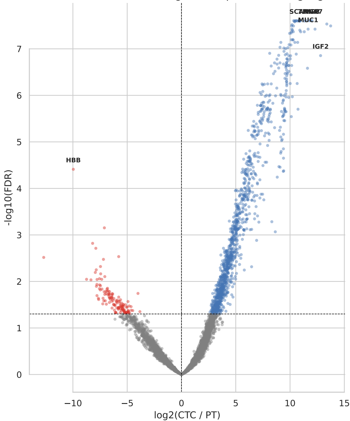
Volcano Plot: CTC vs PT (edgeR) – Paper Genes Highlighted
