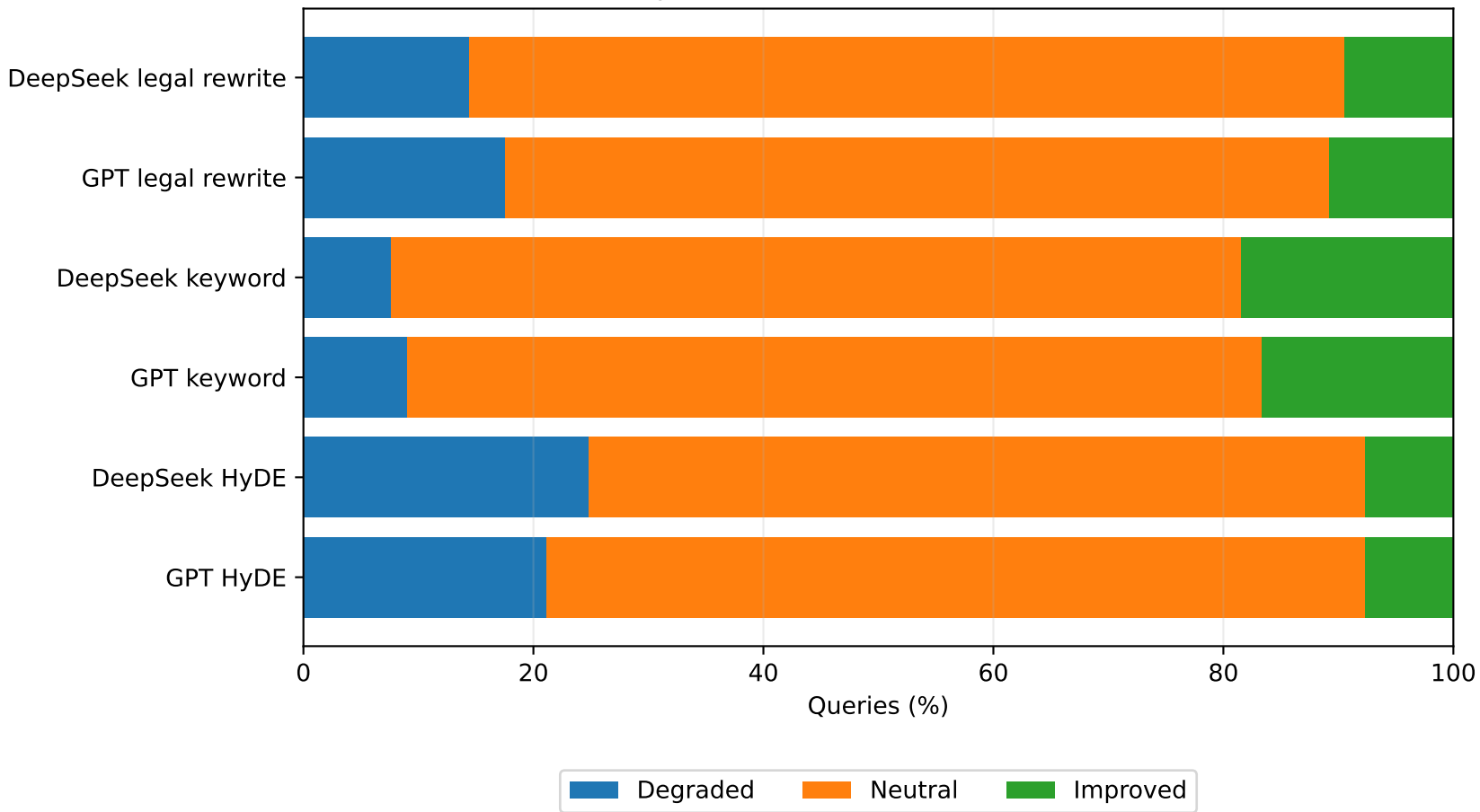
Direct replacement risk on BSARD (Recall@100)
