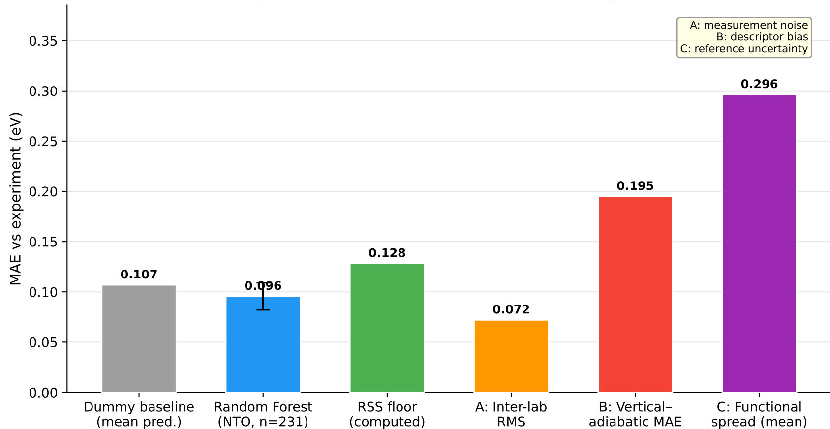
Accuracy ceiling: measured noise components vs model performance
