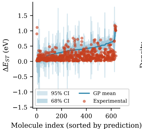
B) Predictions with uncertainty
