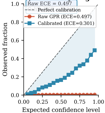
A) Reliability diagram
