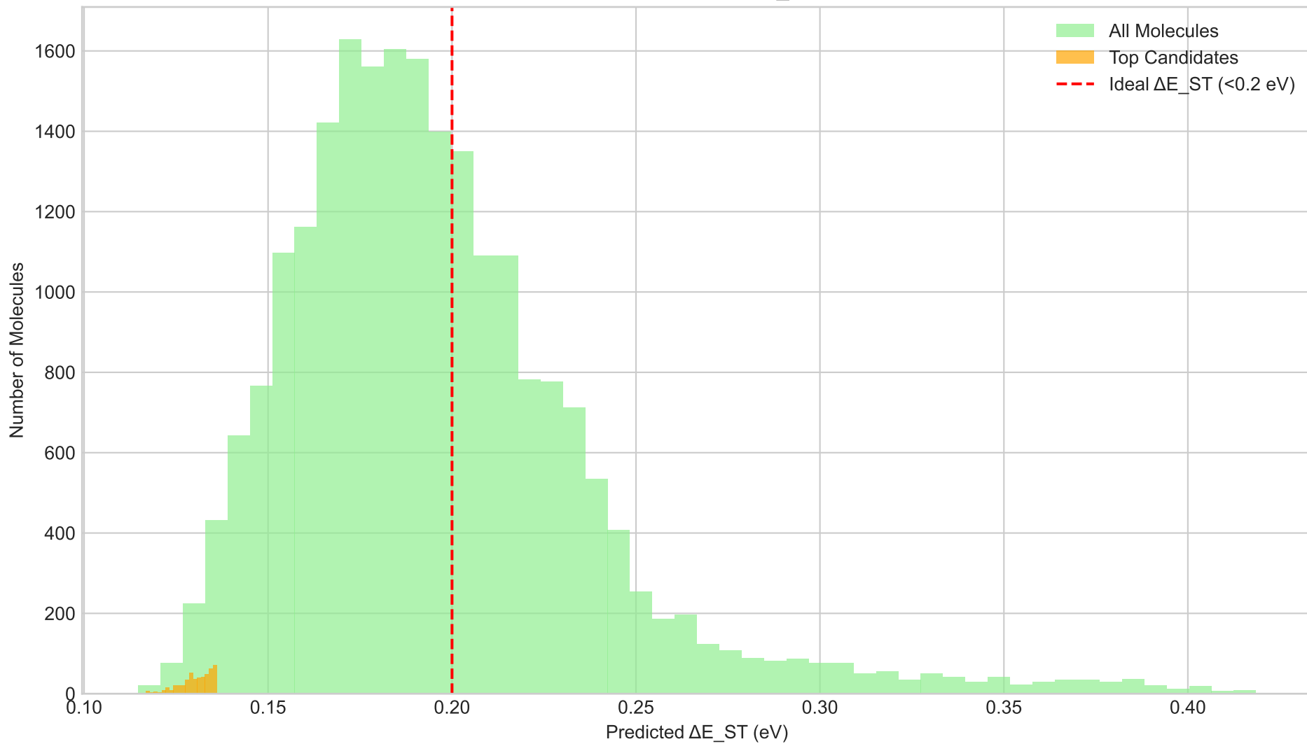
Distribution of Predicted \Delta E_{ST} Values
