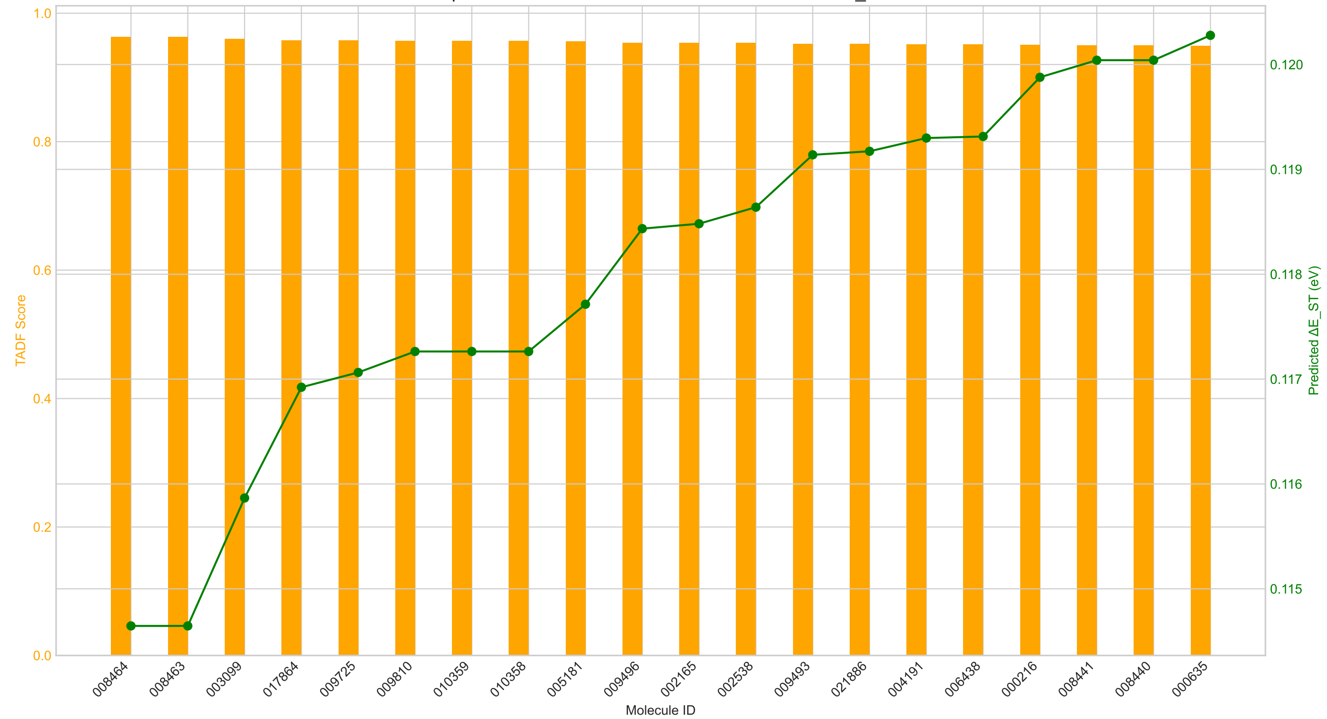
Top 20 TADF Candidates: Scores and Predicted \Delta E_{ST}
