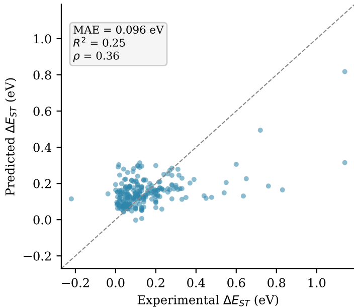
A) Scaffold-CV parity
