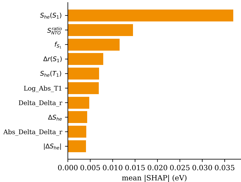
B) Feature importance (RF / SHAP)
