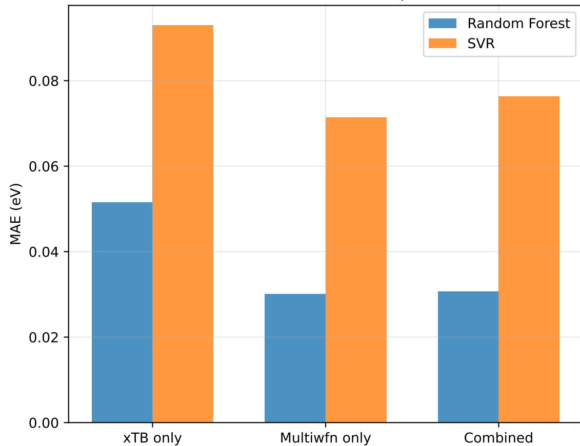
Mean Absolute Error Comparison
