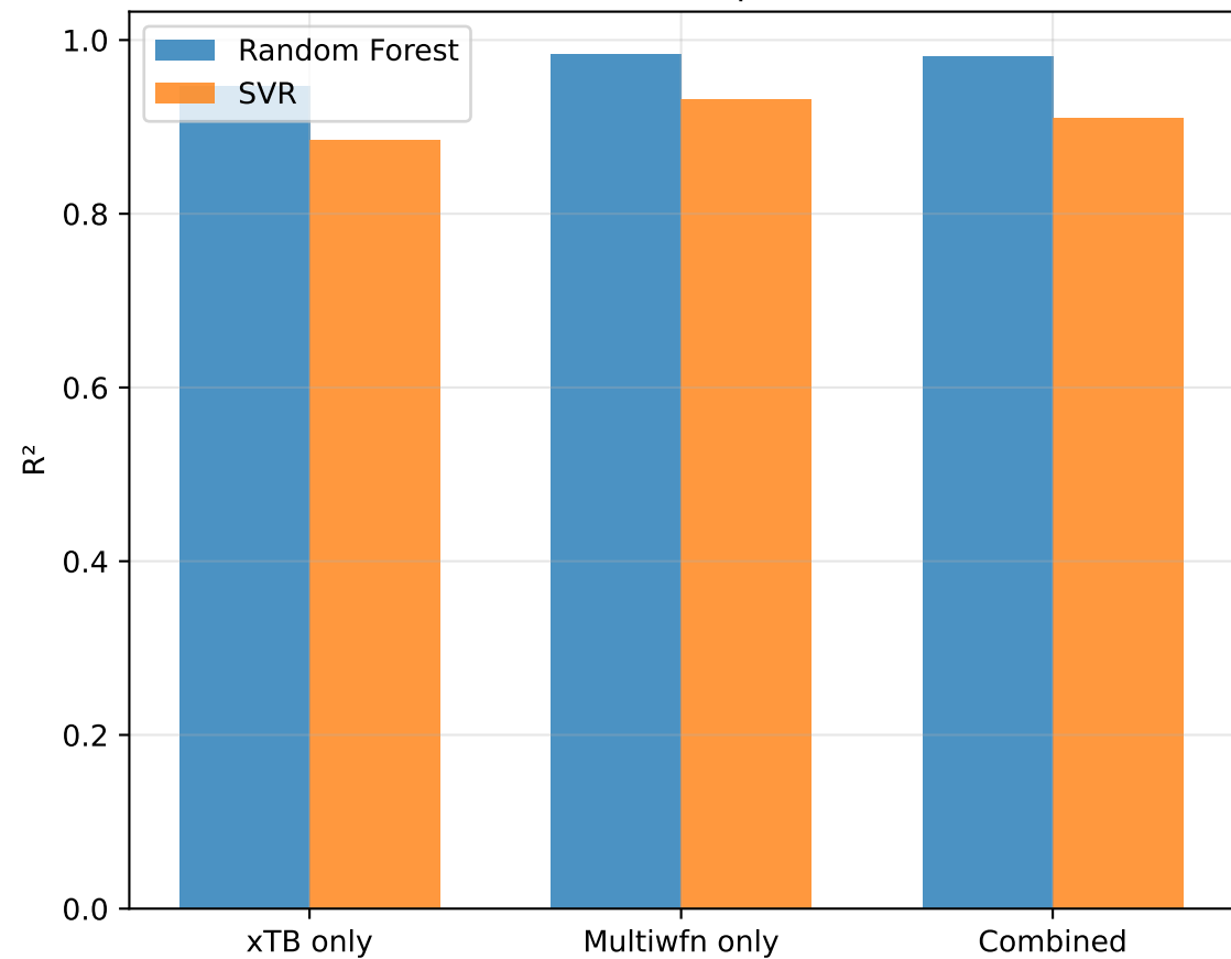
R 2 Score Comparison
