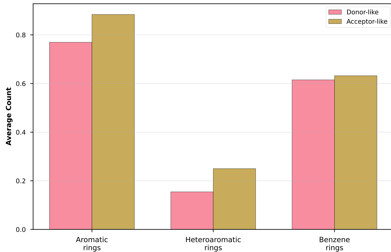
Conjugation & Flexibility
