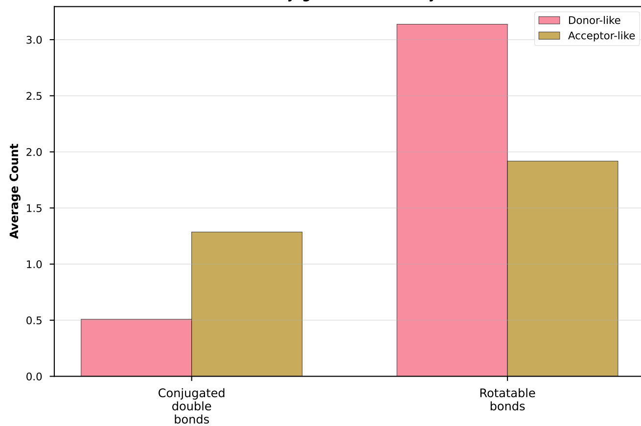
Conjugation & Flexibility
