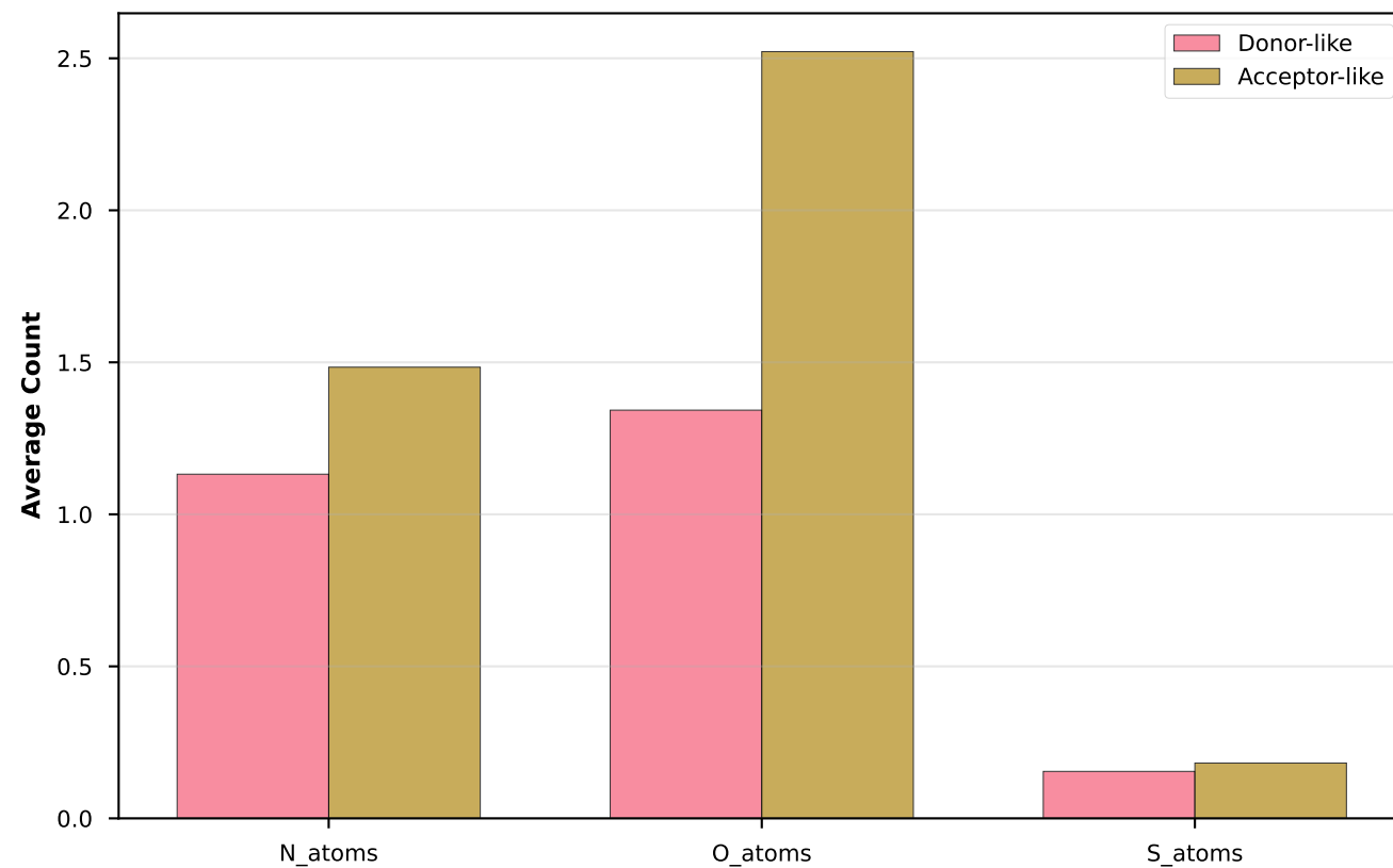
Heteroatom Content
