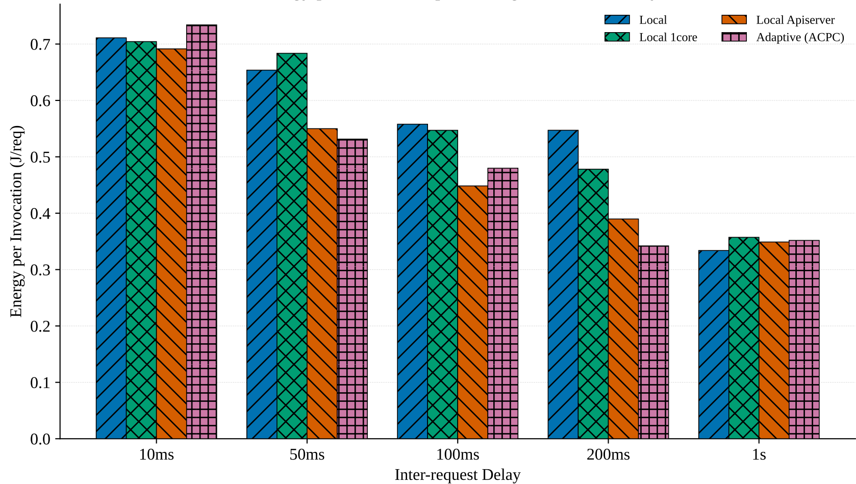
Energy per Invocation per Configuration and Delay
