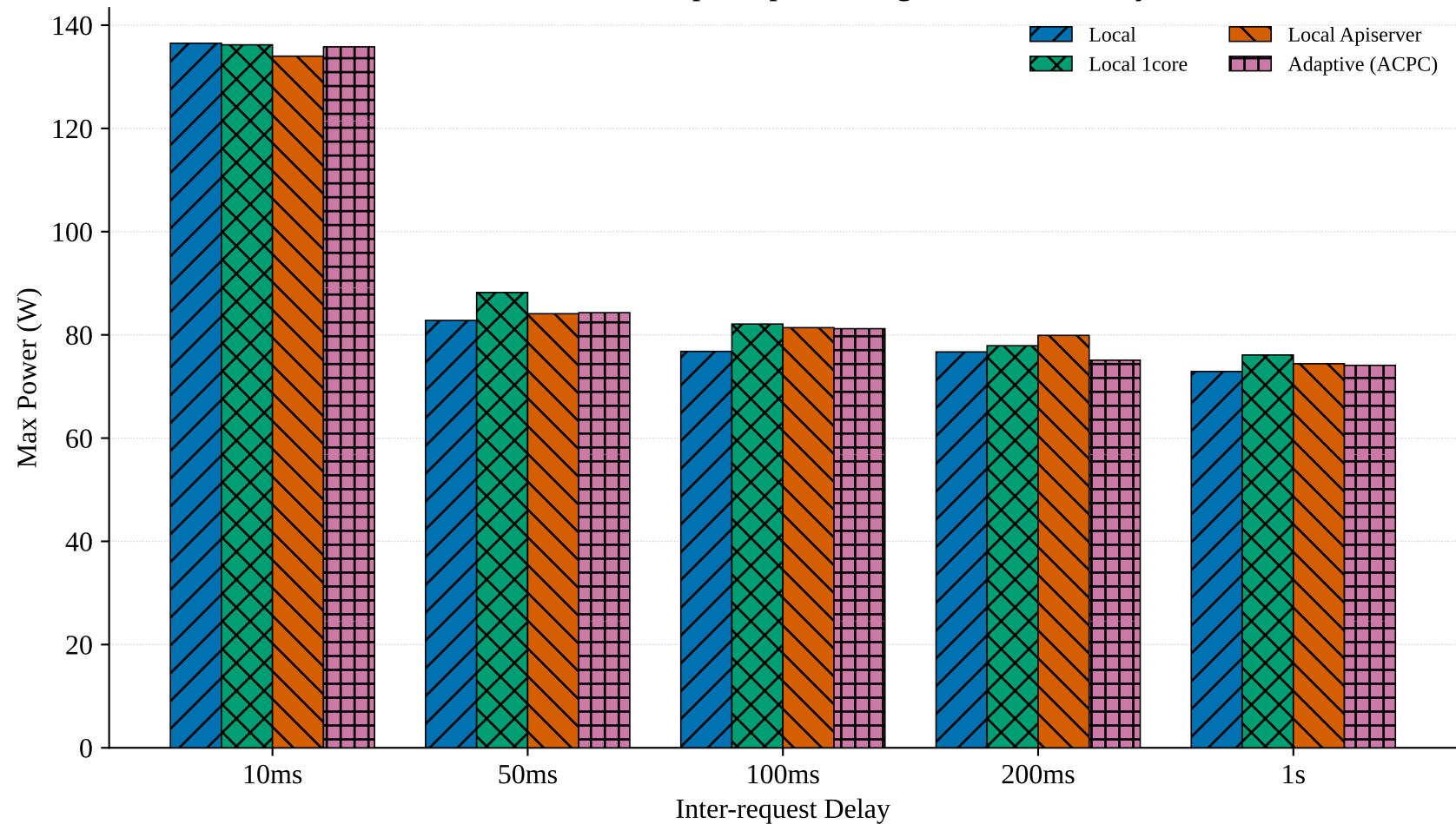
Peak Power Consumption per Configuration and Delay
