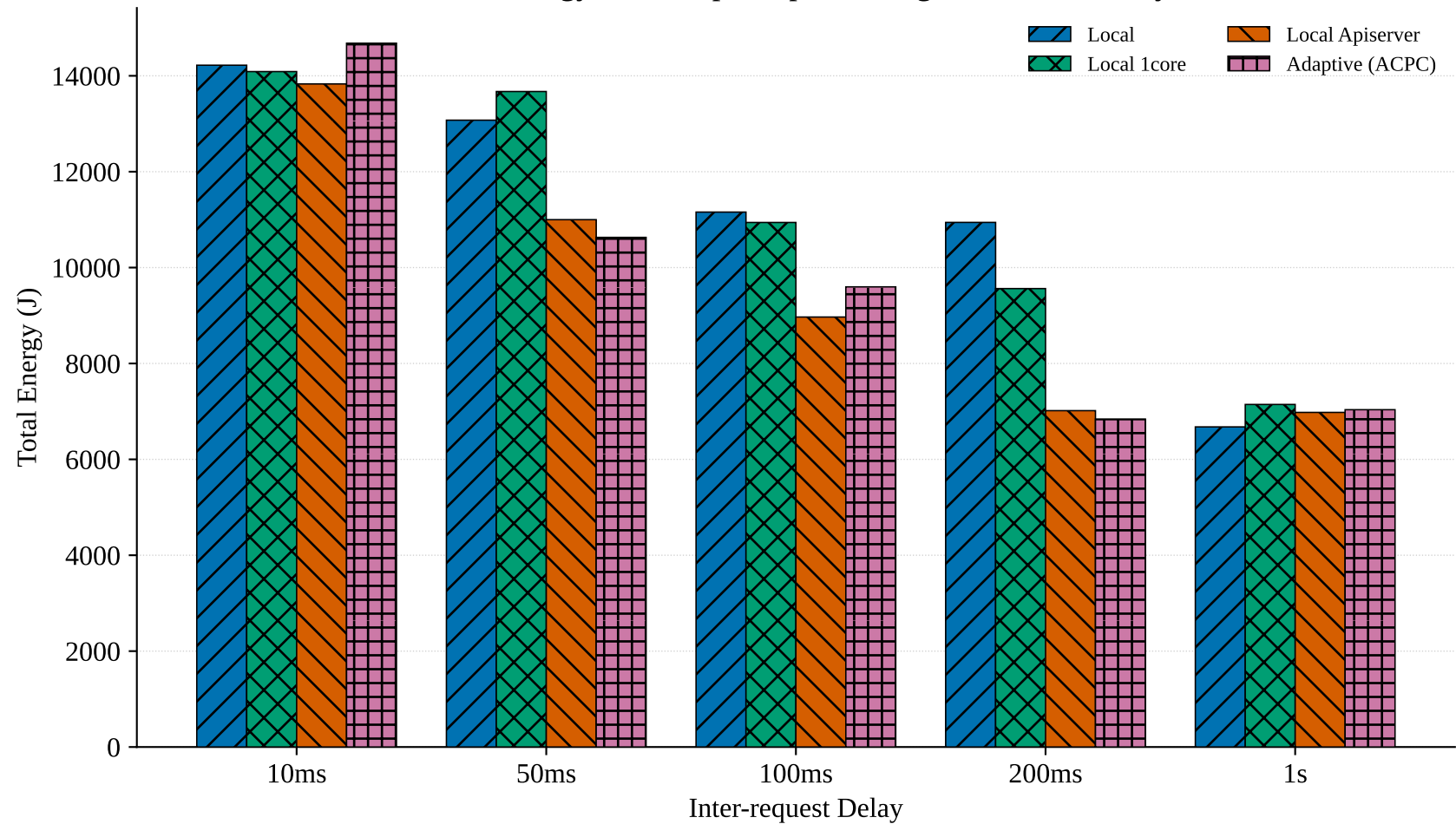
Total Energy Consumption per Configuration and Delay
