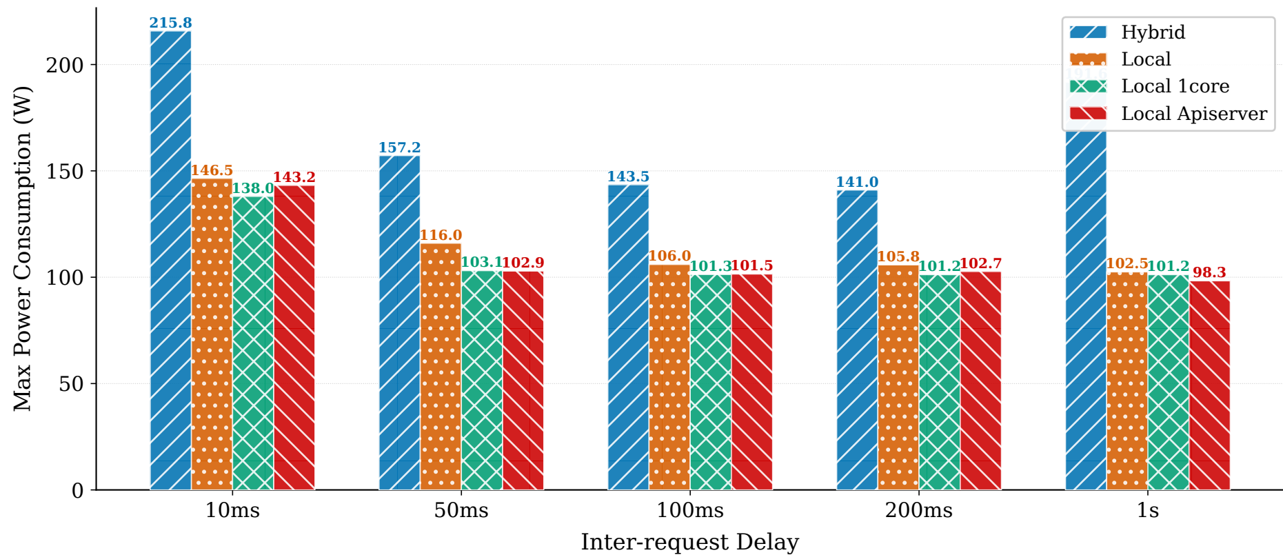
Peak Power Consumption per Configuration and Delay (Maximum observed value) [CPU]
