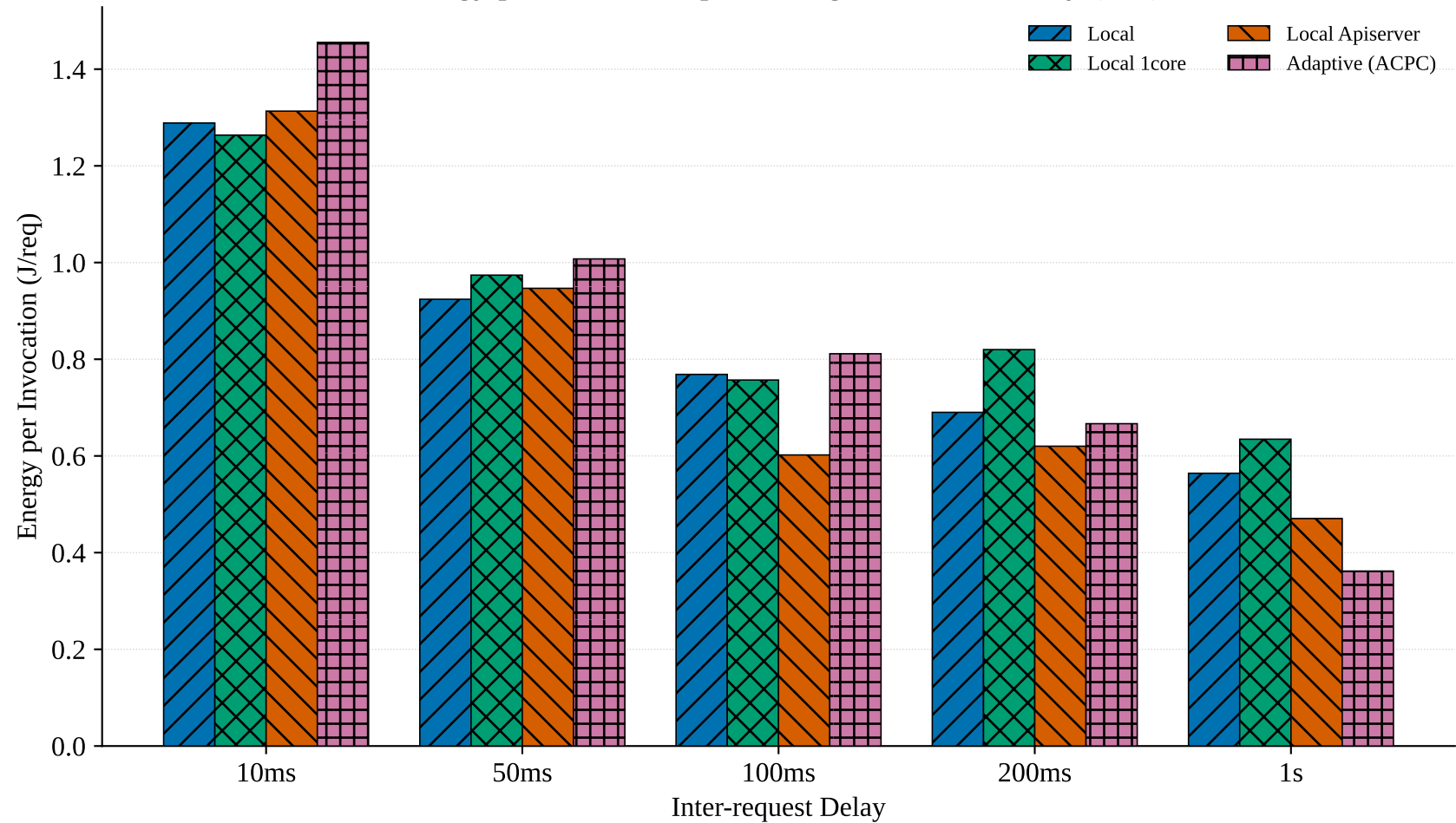
Energy per Invocation per Configuration and Delay (ML)
