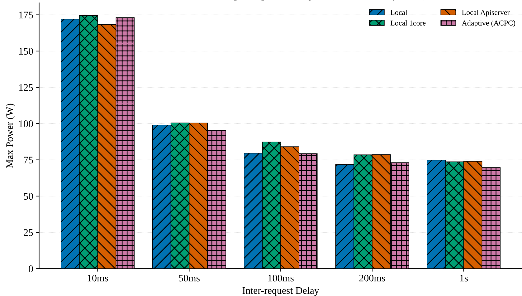
Peak Power Consumption per Configuration and Delay (ML)
