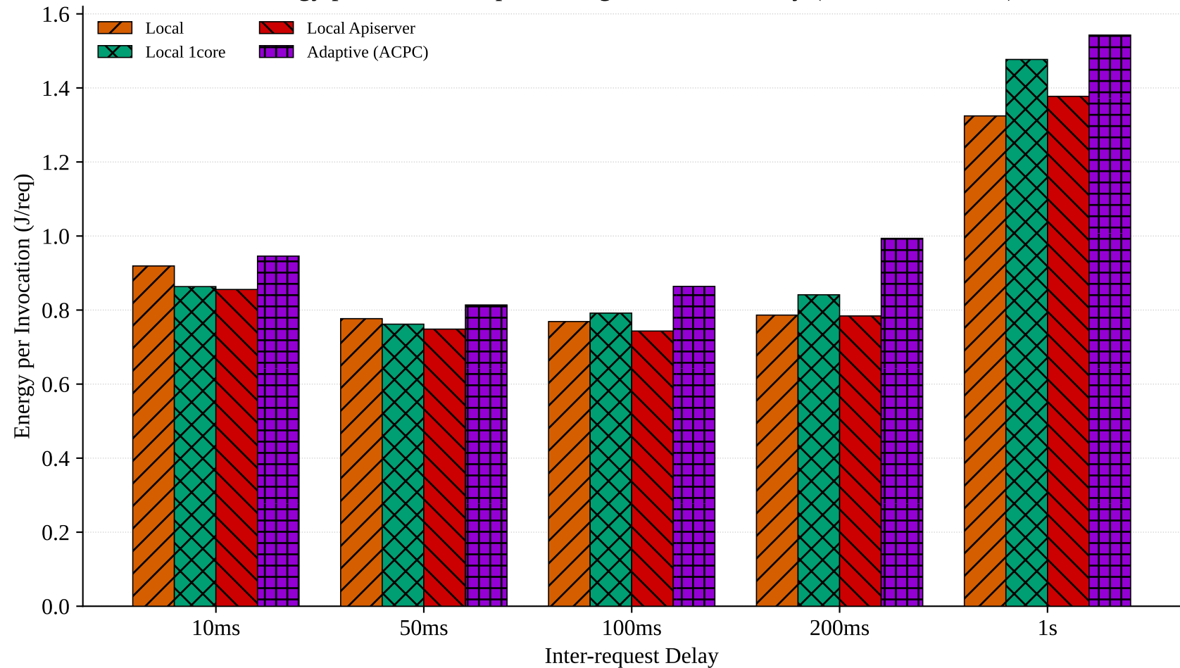
Energy per Invocation per Configuration and Delay (Mixed ML+CPU)
