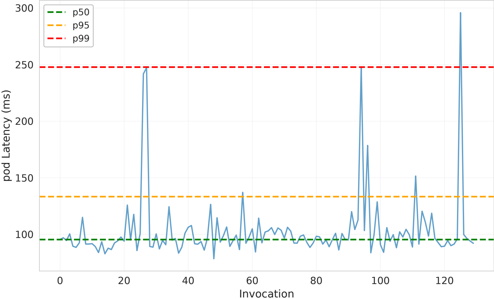
pod Latency — 1s (Local 1 core)
