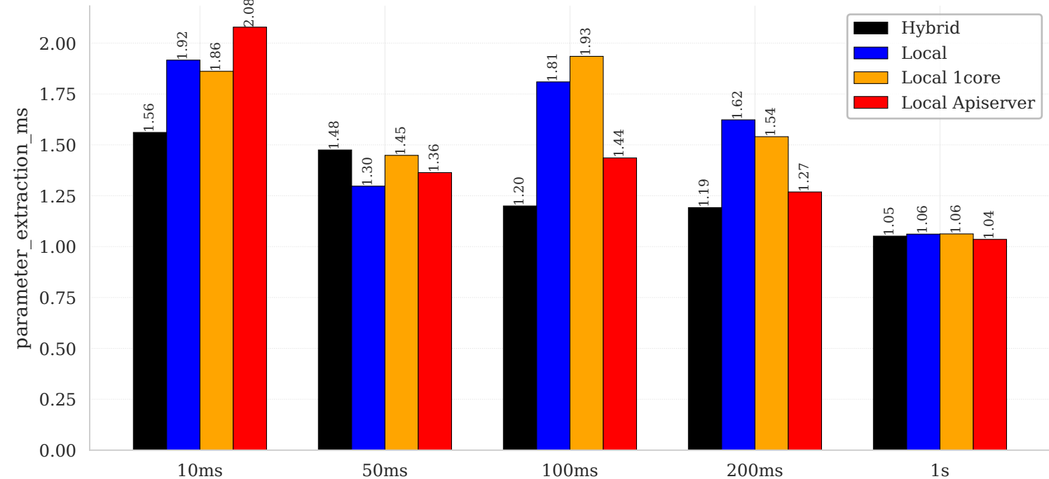
Cold Requests - Parameter Extraction Time
