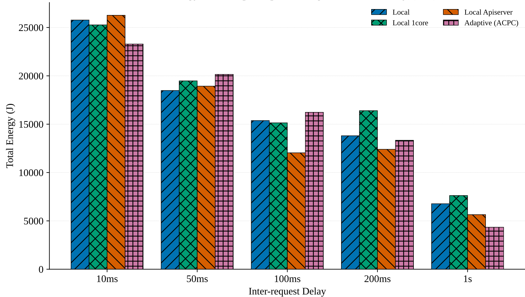
Total Energy Consumption per Configuration and Delay (ML)
