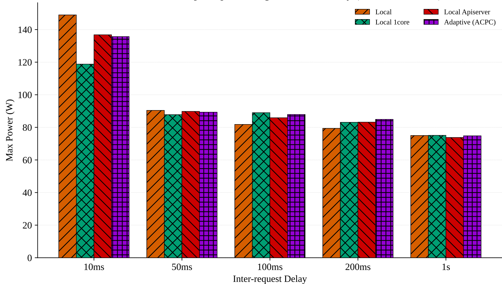
Peak Power Consumption per Configuration and Delay (Mixed ML+CPU)
