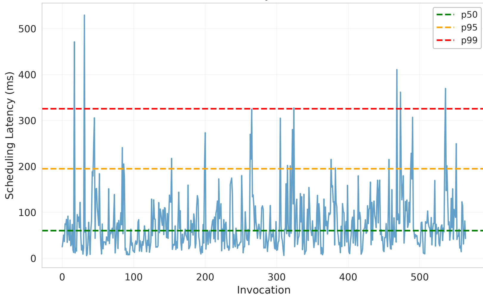
Scheduler Latency — 10 ms Local
