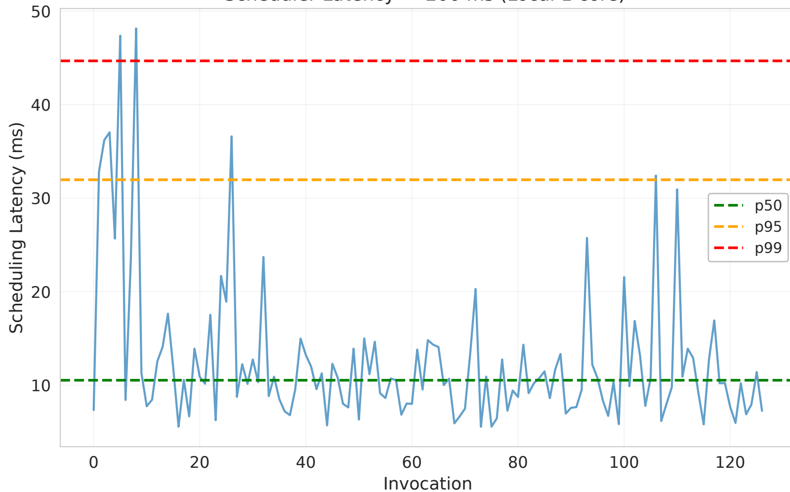
Scheduler Latency — 200 ms (Local 1 core)
