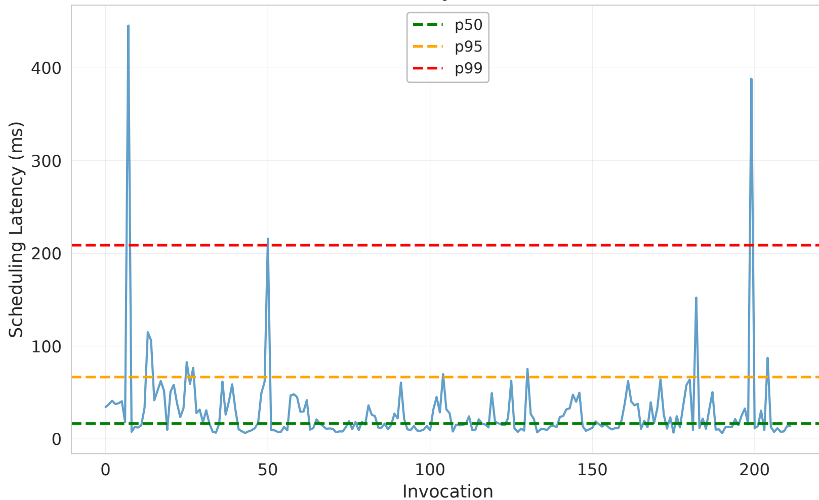
Scheduler Latency — 50 ms (Local)
