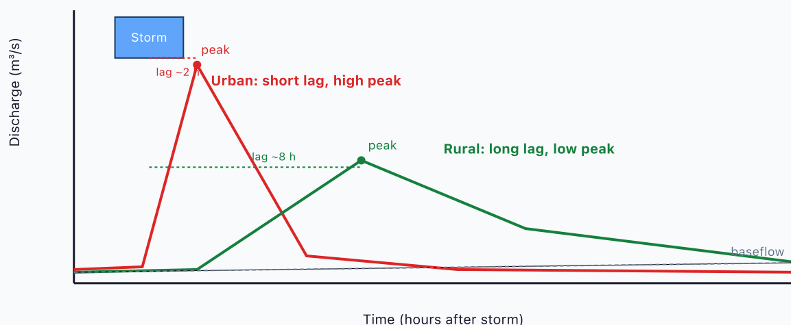
Flood Hydrograph — Urbanised vs Rural Basin Response
