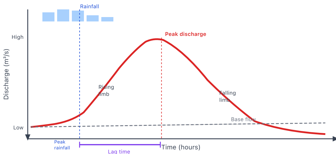
Fig 2.7 — A storm hydrograph showing key components
