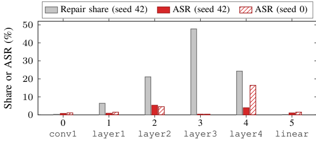
Fig. 1. Per-shard repair share ( \text{share}_s \times 100 , gray) and single-shard rollback ASR under the seed-42 (solid red) and seed-0 (hatched red) repairs, n = 6 . Shard 3 carries the largest share (47.7%) and yields the lowest ASR under both repairs.
