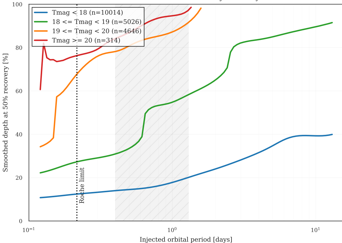
Kernel-smoothed BLS recovery boundary
