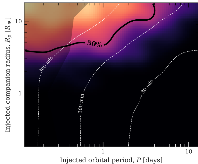
18 &lt;= Tmag &lt; 19: 548/2914 recovered
