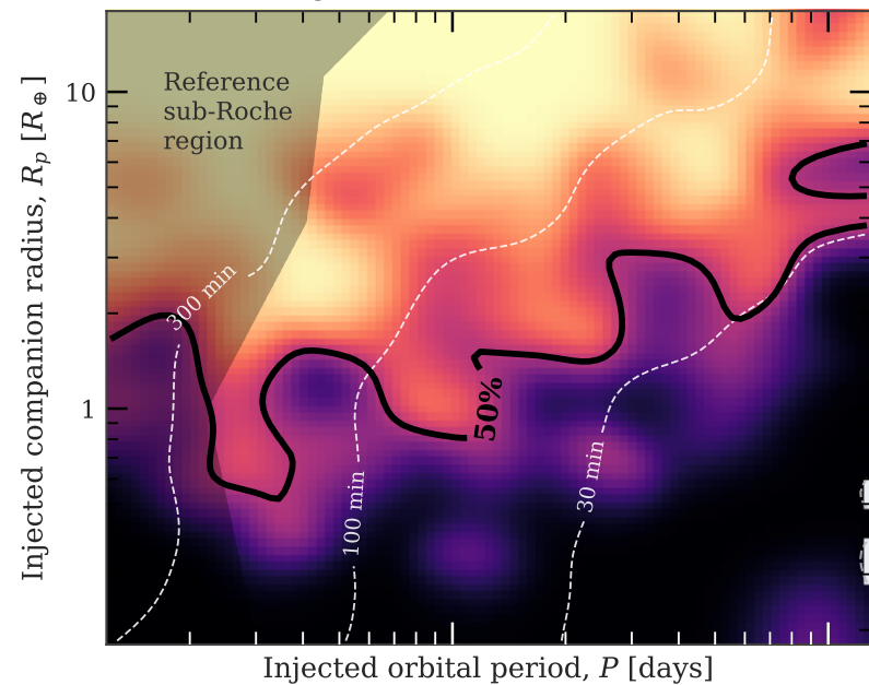
Tmag &lt; 17: 175/324 recovered
