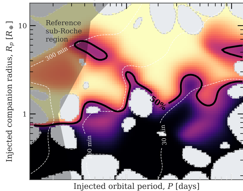
Tmag &lt; 17: 48/88 recovered
