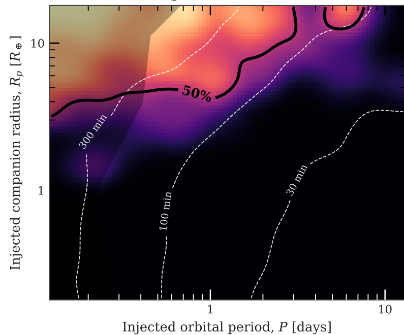
18 &lt;= Tmag &lt; 19: 163/732 recovered
