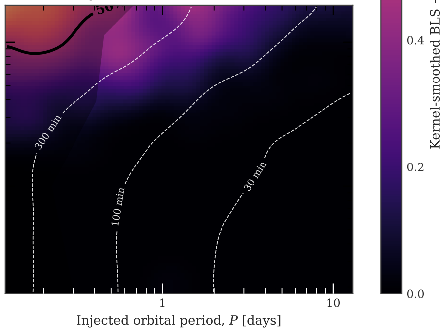
Tmag >= 19: 340/3981 recovered
