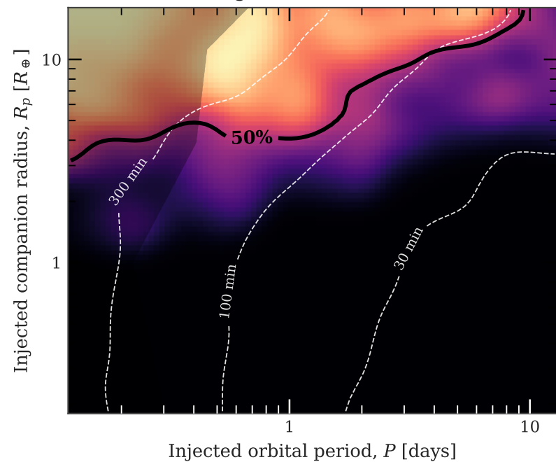
18 <= Tmag < 19: 193/732 recovered
