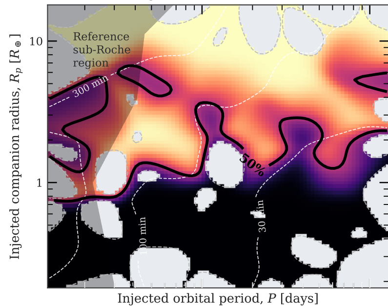
Tmag < 17: 42/88 recovered
