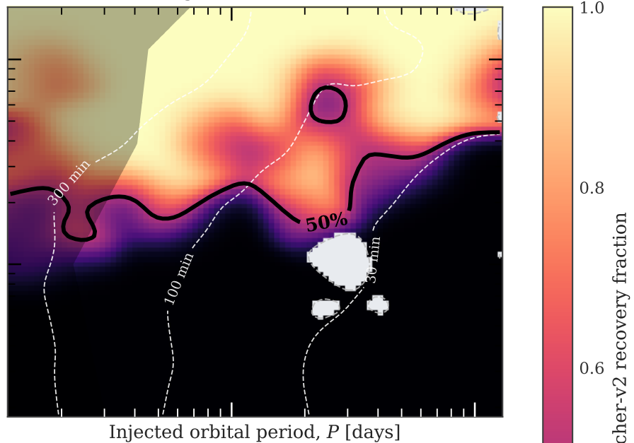
17 <= Tmag < 18: 88/199 recovered
