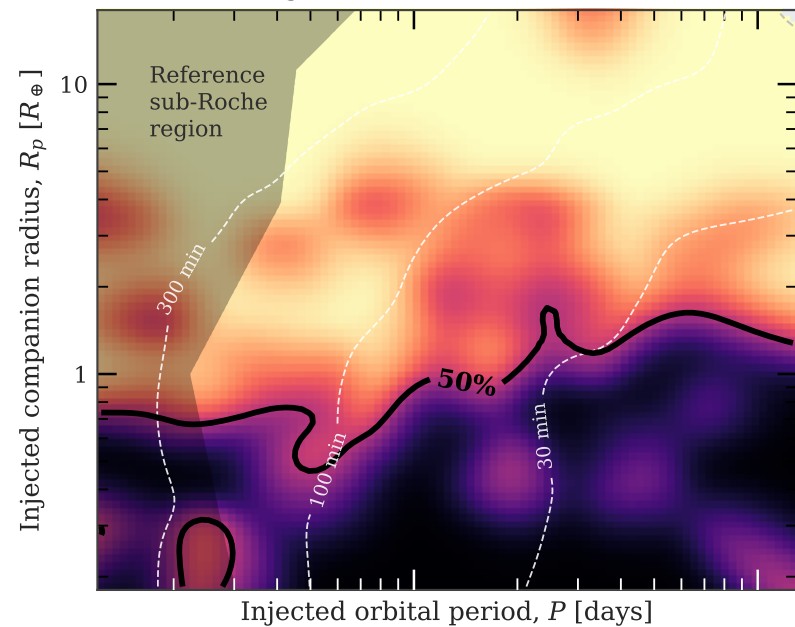
Tmag &lt; 17: 197/303 recovered
