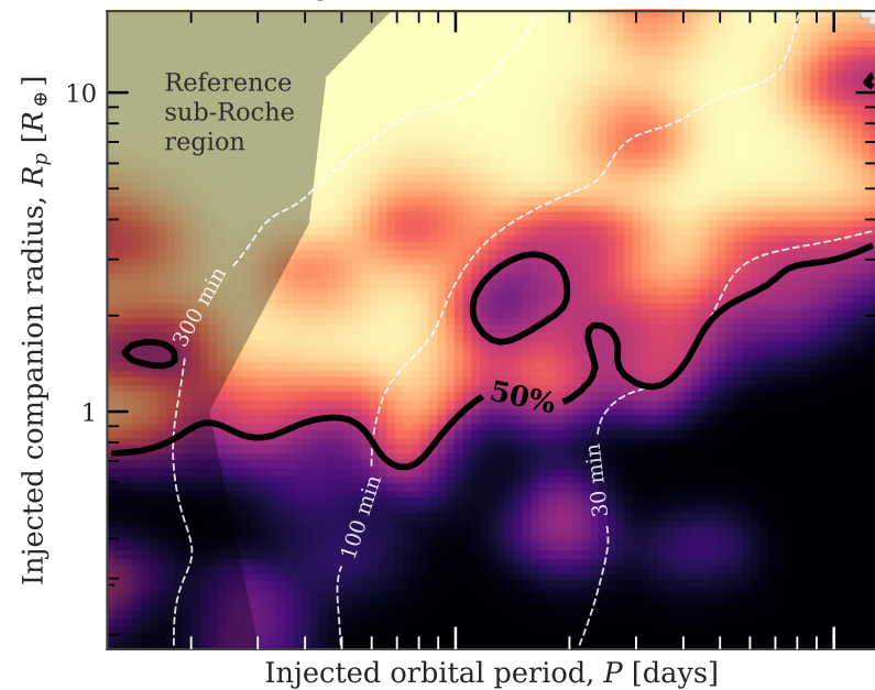
Tmag < 17: 172/303 recovered
