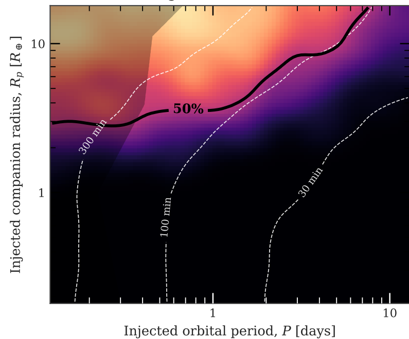
18 <= Tmag < 19: 527/2124 recovered
