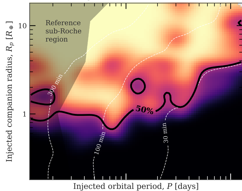
Tmag &lt; 17: 160/303 recovered
