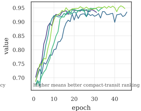
Validation compact AP
