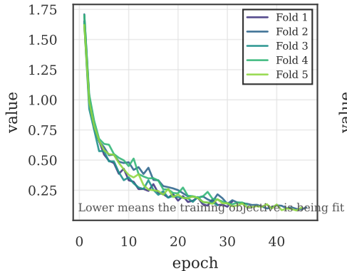
Training loss
