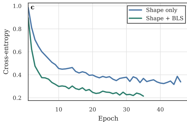
Training loss
