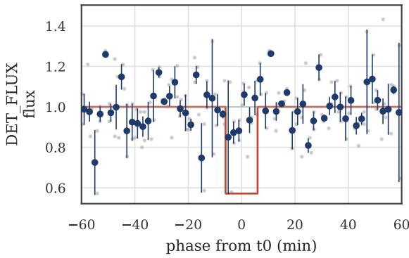
odd/even transit fold (EB check) odd_med=0.315 (n=67) even_med=0.871 (n=68) \Delta=-0.556
