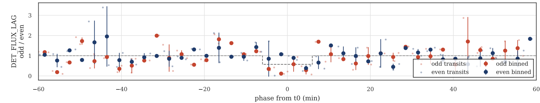
odd/even transit fold (EB check) odd_med=0.315 (n=67) even_med=0.871 (n=68) \Delta=-0.556
