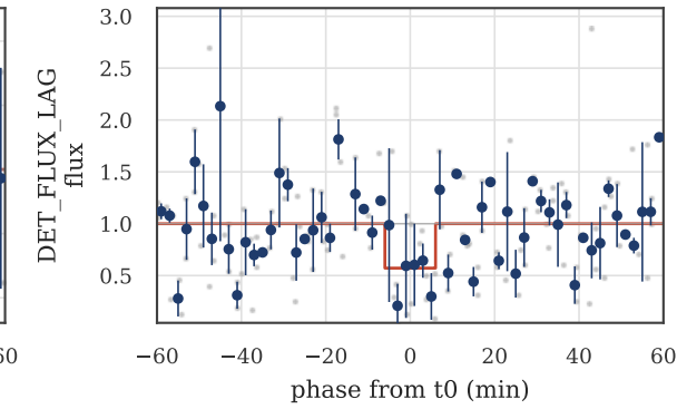
phase fold @ best (P,T0) — DET_FLUX_LAG
