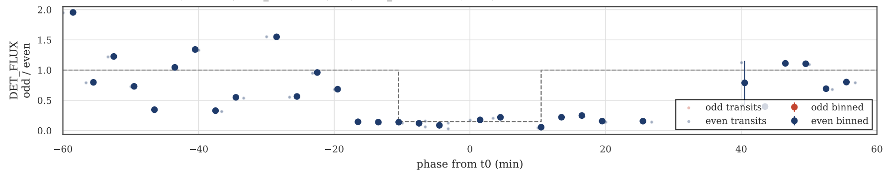
odd/even transit fold (EB check) odd_med=nan (n=0) even_med=0.120 (n=34) \Delta =nan
