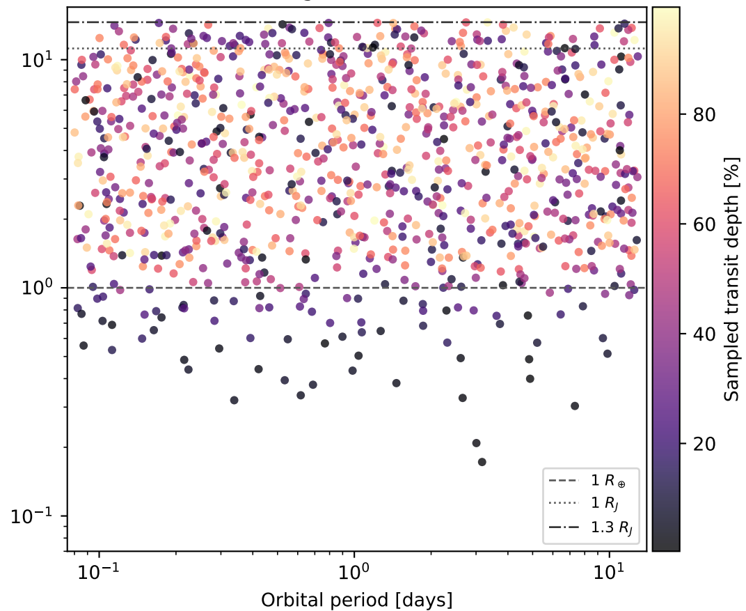
Radius coverage to brown-dwarf scale
