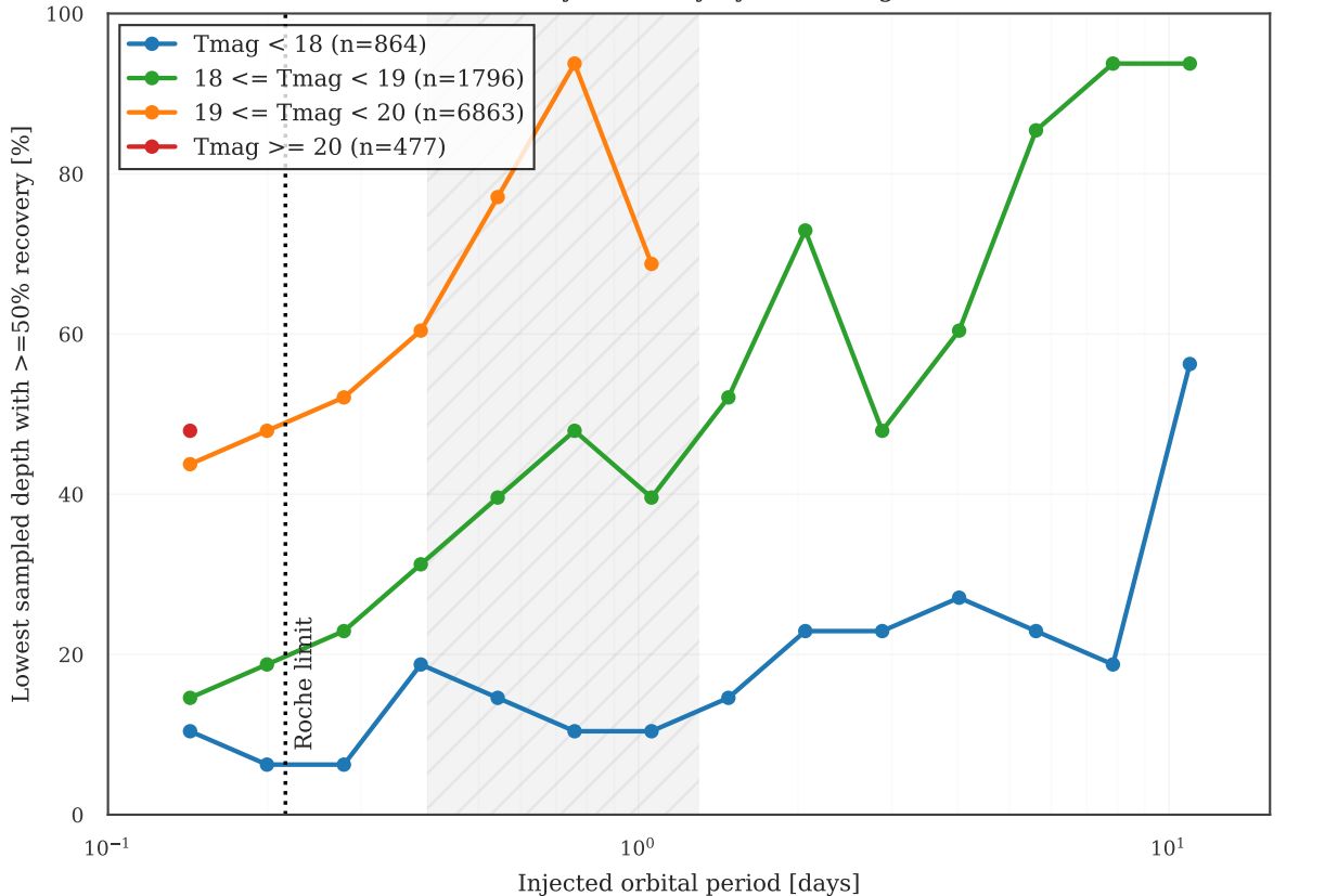
BLS recovery boundary by TESS magnitude
