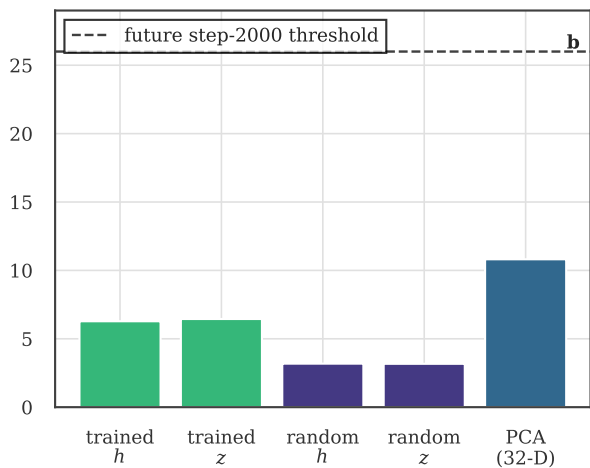
Effective rank
