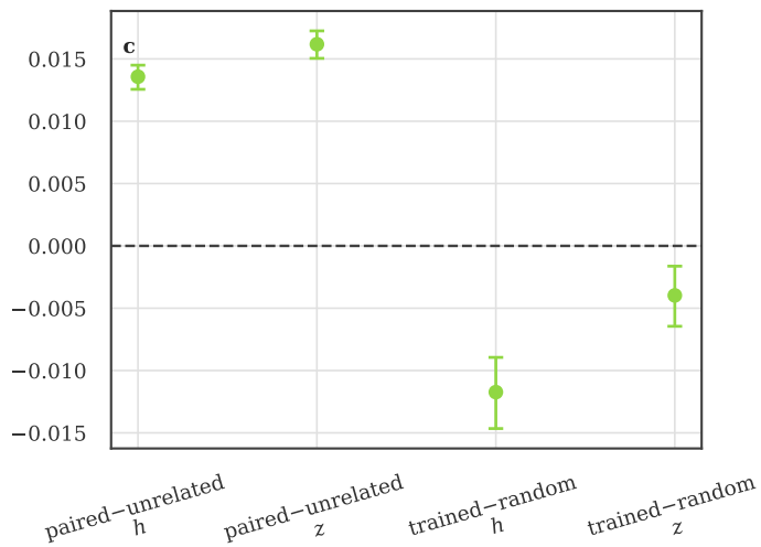
Cosine-similarity difference
