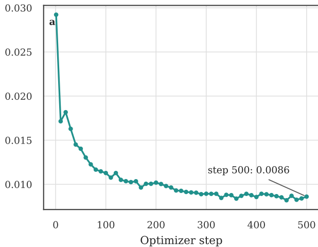
Training objective
