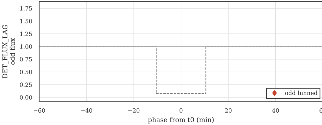
ODD transits @ anchor [DET_FLUX_LAG] med=nan n=0
