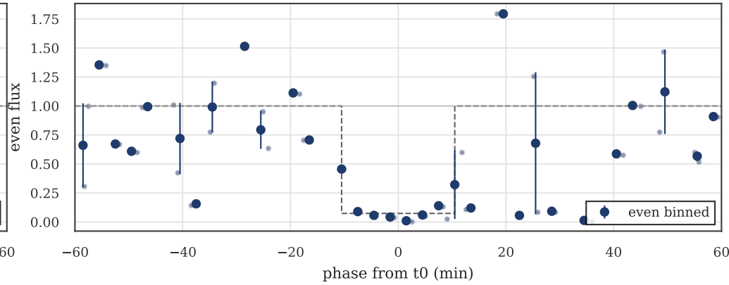
EVEN transits @ anchor [DET_FLUX_LAG] med=0.060 n=39
