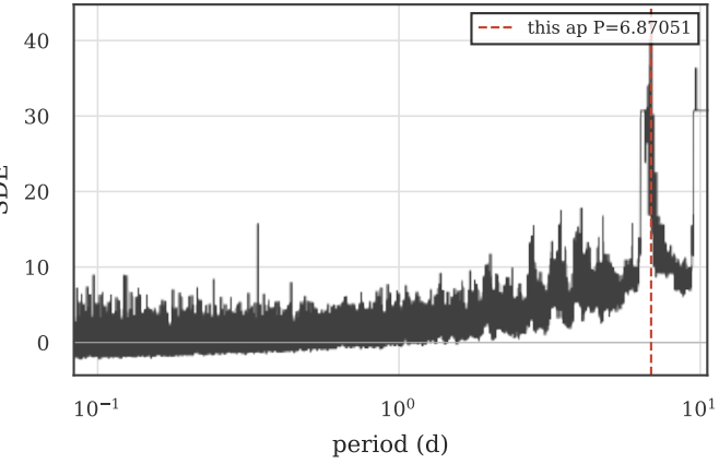
DET_FLUX_LAG fold @ own P=6.87051 d (SDE=42.5)
