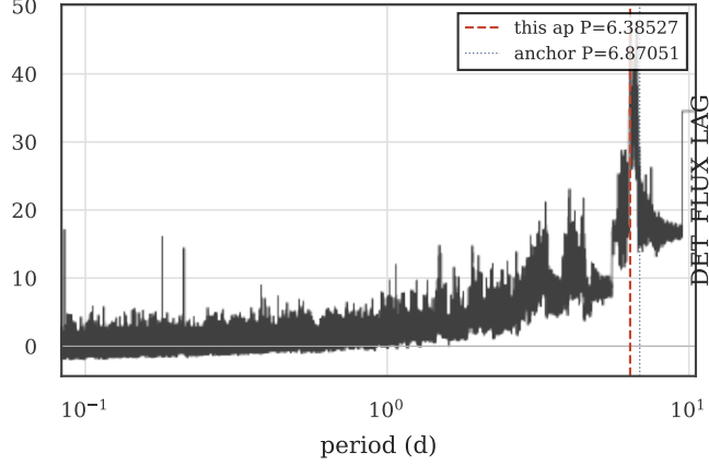
DET_FLUX fold @ own P=6.38527 d (SDE=47.7)
